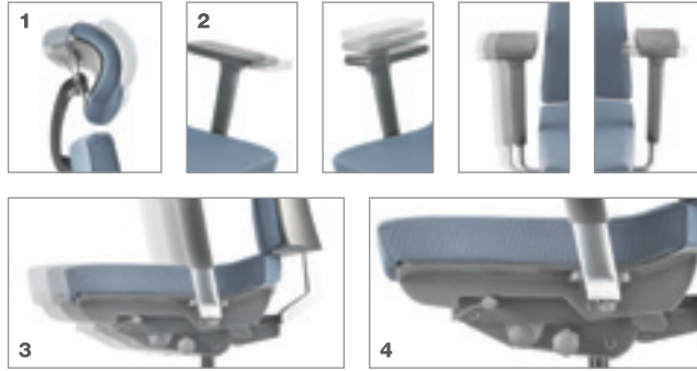
1. Adjustable Headrest
